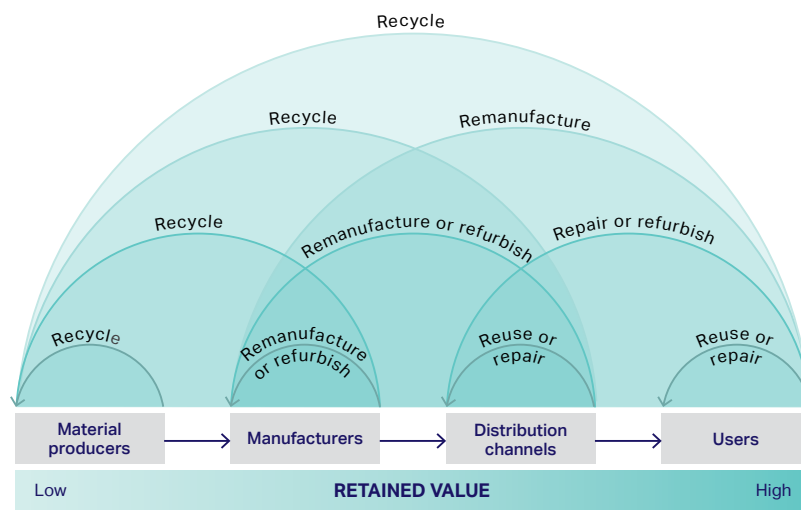
Figure 9: Retained value
